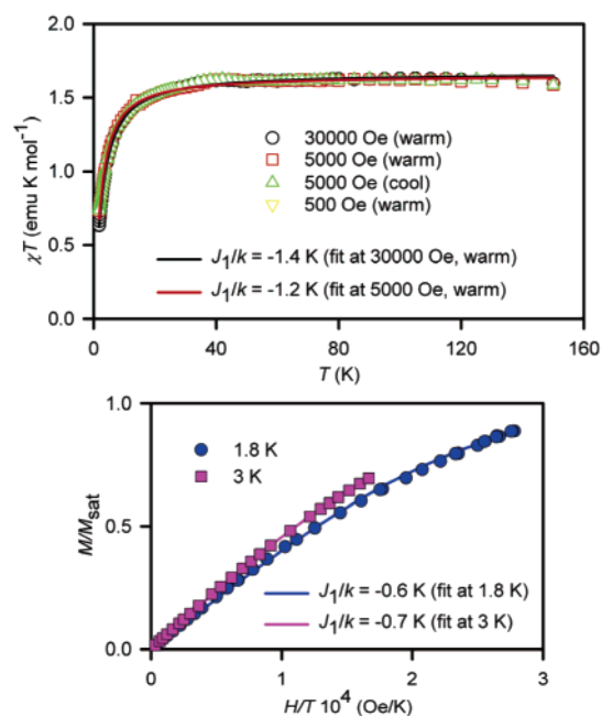
Figure 8. SQUID magnetometry for 5 mM 1 in THF with numerical fits to the tetradical model (Figure 10, eqs 1 and 2). For the \chi T versus T fits (top) and the M/M_{\text{sat}} versus H/T fits (bottom), the J_2/k (diagonal coupling) is set to -1.1 and -0.5 K, respectively. The variable parameters (parameter dependence and R^2 ) are as follows: at 30 000 Oe in the warming mode, J_1/k = -1.4 K, w = 1.11 (0.32, 0.998); at 5000 Oe in the warming mode, J_1/k = -1.2 K, w = 1.10 (0.30, 0.995); at 1.8 K, J_1/k = -0.6 K, M_{\text{sat}} = 0.76 \mu_{\text{B}} (0.85, 0.999); at 3 K, J_1/k = -0.7 K, M_{\text{sat}} = 0.86 \mu_{\text{B}} (0.97, 1.000).
