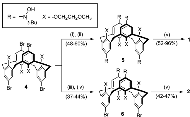
Scheme 1. Synthesis of Nitroxide Tetradical 1 and Diradical 2 a
