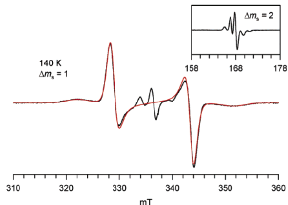
Figure 7. EPR (X-band, 9.4424 GHz) spectrum of 0.6 mM nitroxide diradical 2 in toluene/chloroform (4:1) at 140 K. The spectral simulation of the |\Delta m_{\text{S}}| = 1 region is shown as red trace. The fitting parameters for the spectral simulation for the S = 1 state are: |D/hc| = 1.39 \times 10^{-2} \text{ cm}^{-1} ( |D/g\mu_{\text{B}}| = 14.9 mT), |E/hc| = 0 \text{ cm}^{-1} , g_{\text{x}} = 2.0064 , g_{\text{y}} = 2.0064 , g_{\text{z}} = 2.0030 , Gaussian line ( L_{\text{x}} = 12 G, L_{\text{y}} = 20 G, L_{\text{z}} = 40 G). The center lines correspond to an S = 1/2 (monoradical) impurity.
